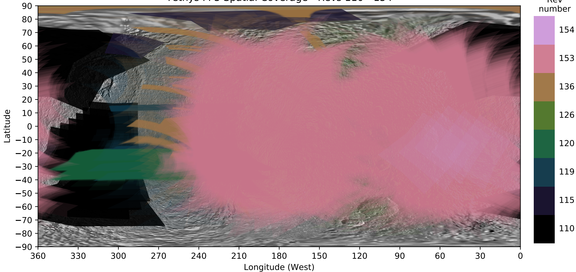
Tethys FP3 Spatial Coverage - Revs 110 - 154
