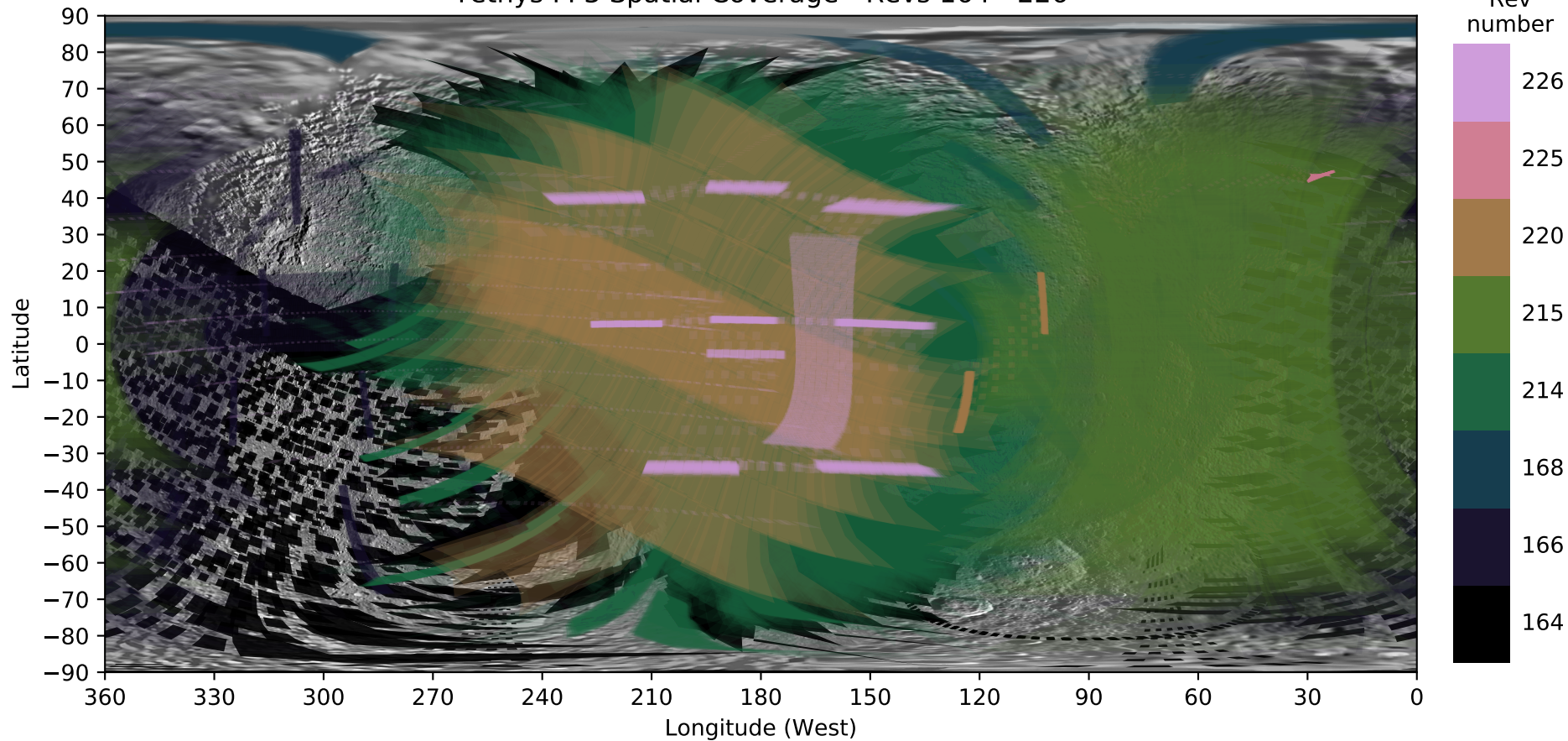
Tethys FP3 Spatial Coverage - Revs 164 - 226
