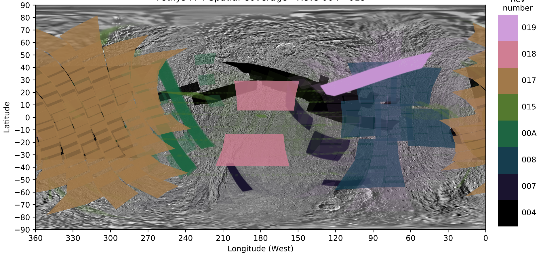
Tethys FP4 Spatial Coverage - Revs 004 - 019
