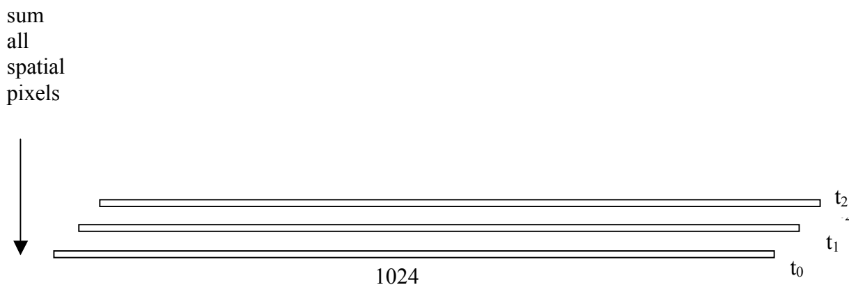
Figure 2.1C: A series of spectra.
