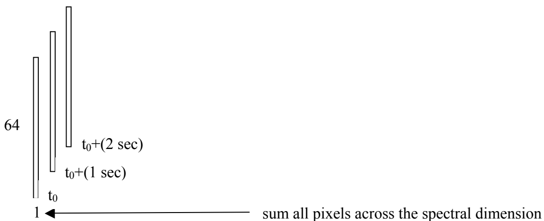
Figure 2.1B: An image at one wavelength
