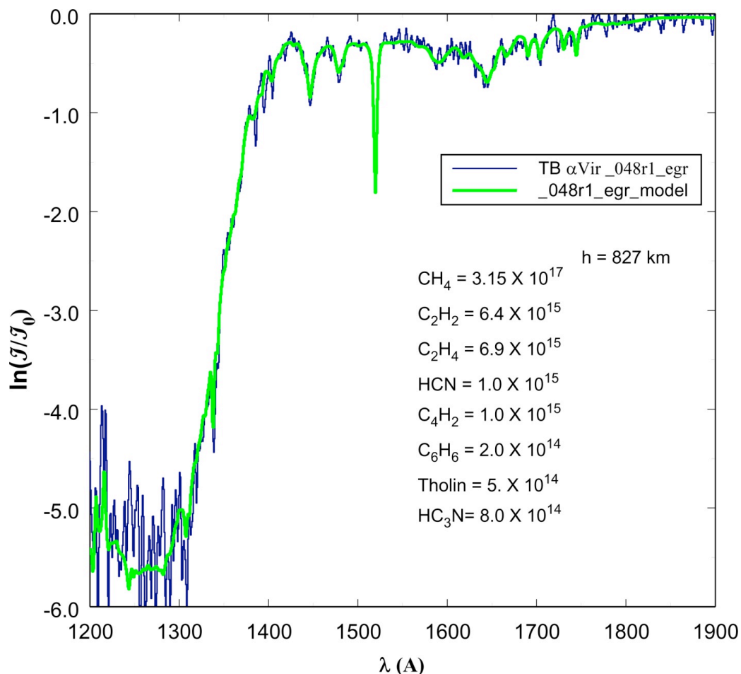
Figure 10.2: Occlusion extinction spectrum of \alpha Vir at Titan TB encounter against model calculations for an impact parameter altitude of 827 km. Figure 10.1 is a long wavelength component of this spectrum. The fully developed model is shown in green. The species \text{CH}_4 , \text{C}_2\text{H}_2 , and \text{C}_2\text{H}_4 are built into the model at a temperature of 150 K. Signal noise is evident at an optical depth of 6.
