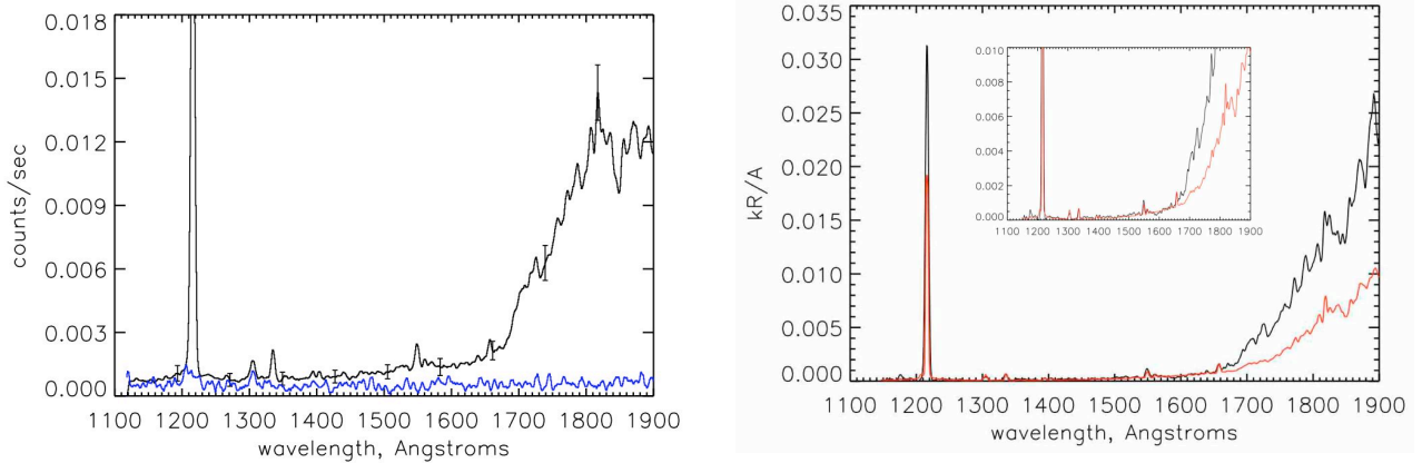
Figure 8.3. Sample spectra from Phoebe (phase angle \alpha = 42^\circ ). (left) Average raw spectrum (counts/s) from the dayside (average of 1224 spectra) and nightside background spectrum (in blue), with sample 1- \sigma statistical error bars shown. (right) Average calibrated spectrum (kR/Å), nightside background subtracted, with scaled solar spectrum overplotted (in red). The solar spectrum has been scaled by fitting to the reflected 1335 Å C II feature in the Phoebe spectrum.
