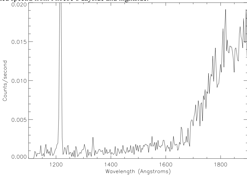
Figure 1.2: 2004 UVIS observation of Phoebe's dayside.
