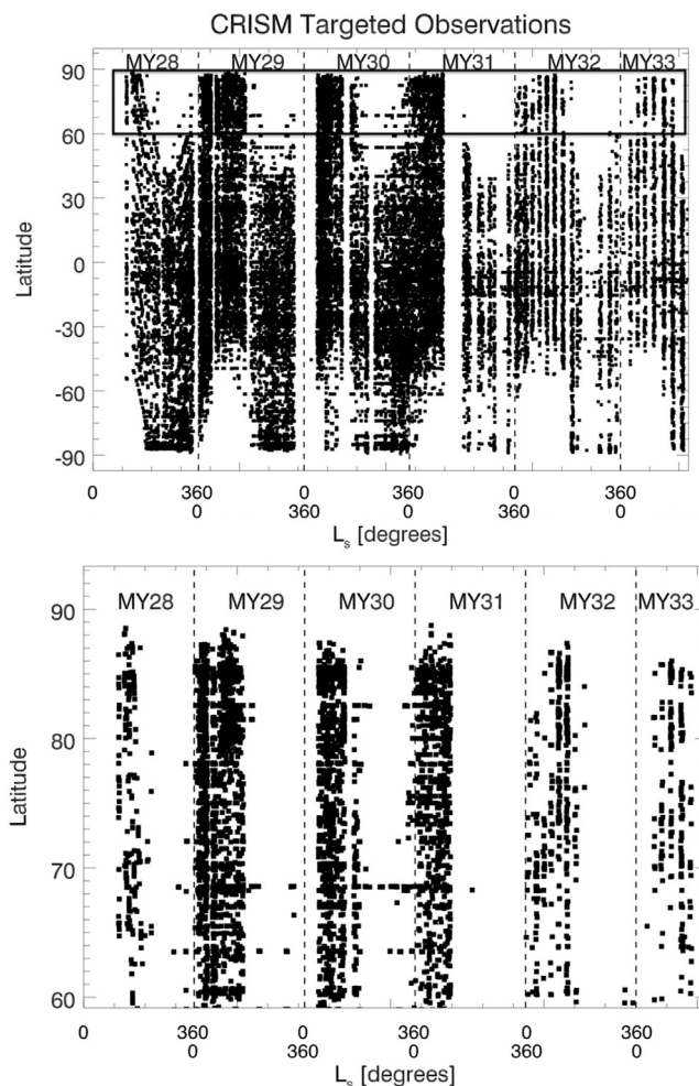
Fig. 1. The seasonal ( L_s ) and latitudinal distribution of the CRISM observations used in this work. The top panel represents the CRISM targeted observations across the Martian globe, whereas the bottom panel represents a subset of the targeted observations, over latitudes higher than 60^\circ\text{N} . L_s = 0^\circ\text{--}360^\circ corresponds to one Mars Year (MY). The gaps near the winter poles are due to the limitations on the solar incidence angle. We made use of the observations over the NPC from the bottom panel to characterize the water cycle over the polar cap, and to link them to the global observations from the top panel to measure the meridional water transport between the NPC and lower latitudes.
