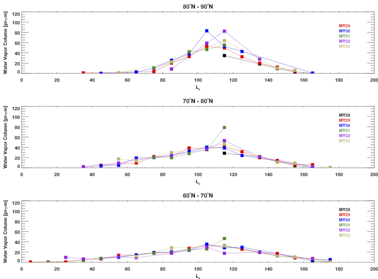
Fig. 11. The seasonal evolution of the atmospheric water vapor column abundance (pr- \mu\text{m} ) in three different latitude bands in the north polar region, for the Martian years as observed by CRISM. The different colors represent the different Martian years.
