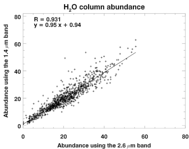
Fig. 6. The scatter plot obtained by plotting the retrieved water vapor abundances using the modified version of the radiative transfer model that relies on the water vapor band at 1360\text{ nm} and which uses weighting factors, against the retrievals from using the water vapor band at 2600\text{ nm} . The Pearson correlation coefficient found is 0.93 .
