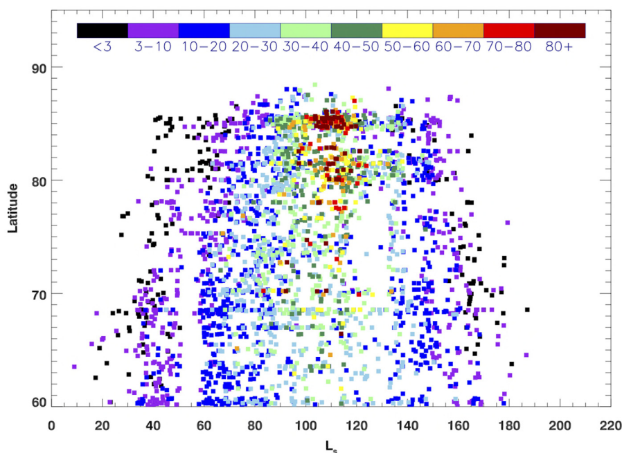
Fig. 8. The variation of the atmospheric water vapor column abundance ( \text{pr-}\mu\text{m} ) during northern spring and summer as a function of latitude from the combined Mars Years (MY 28 to MY 33), as retrieved from \sim 2700 CRISM spectra taken over the north polar region.
